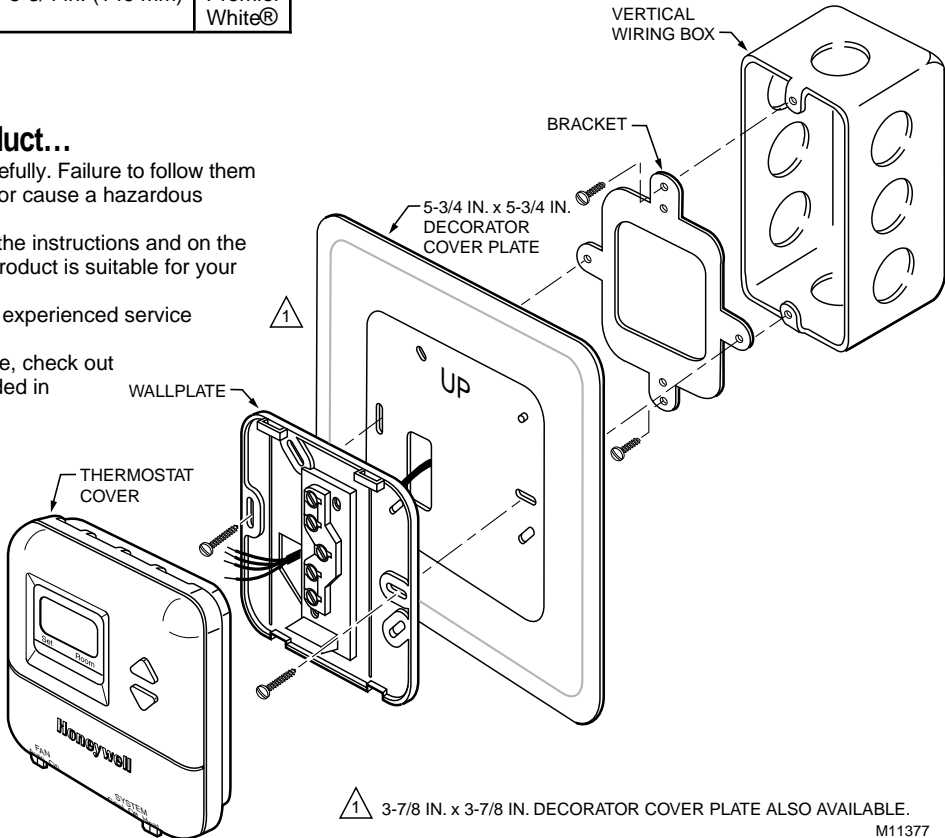
Fig. 1. Mount thermostat, wallplate, cover plate and bracket to wiring box.
