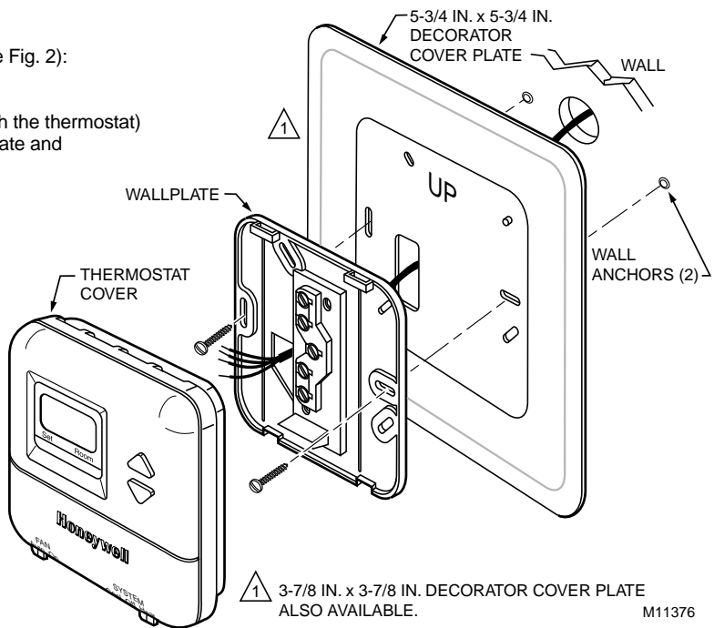
Fig. 2. Mount thermostat, wallplate, and cover plate to wall.
